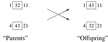
Fig. 14. Crossover 2 – subsequence exchange for ordinal number encoding
